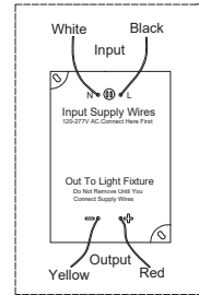
Wiring diagram
